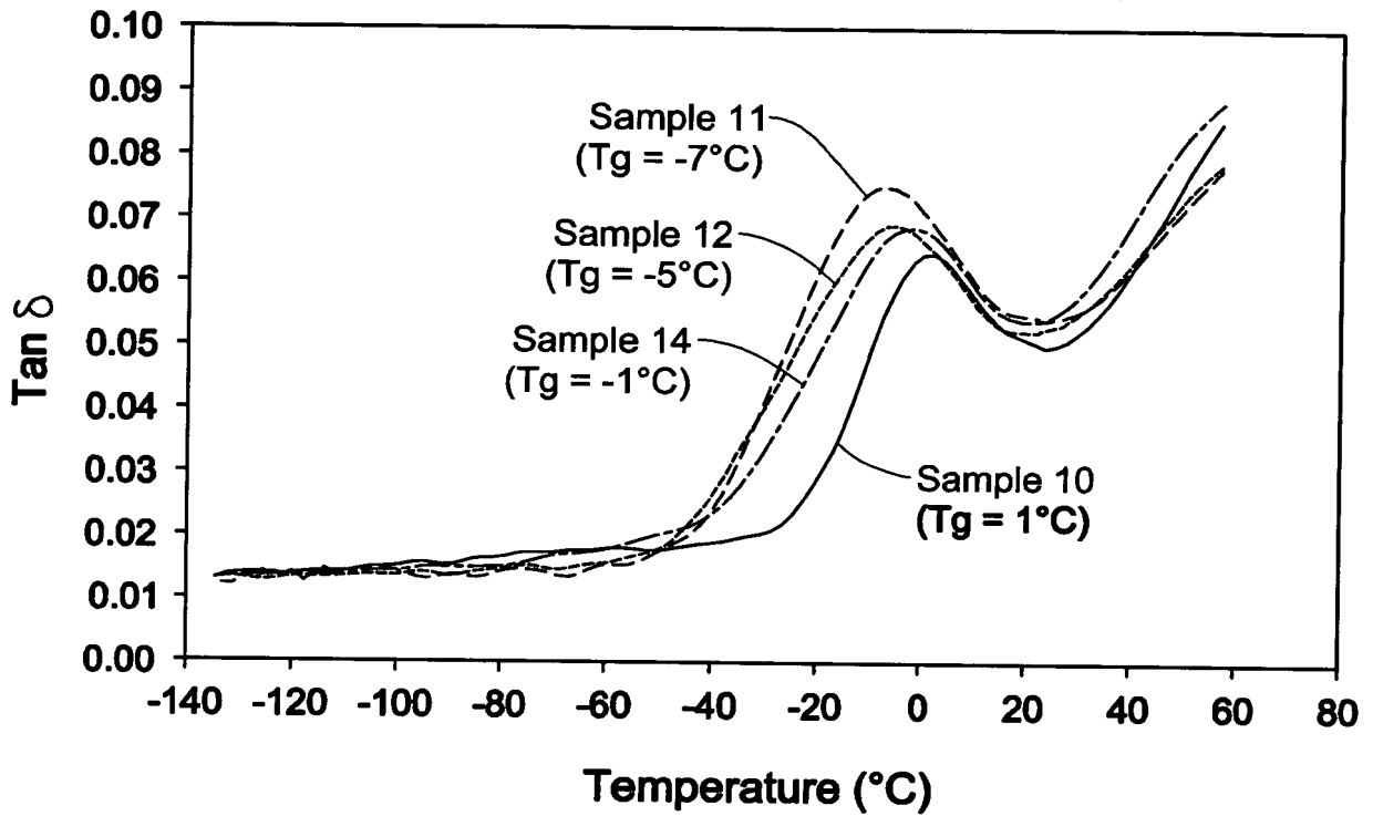
Fig. 3 Tan \delta of Plasticized Propylene Copolymers
